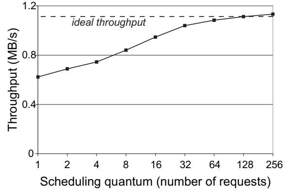
Figure 11: Effect of scheduling quantum on throughput.
