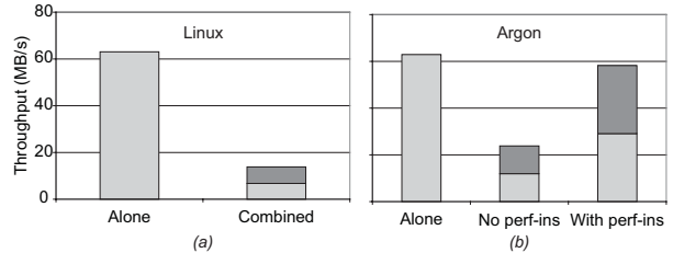
Figure 3: Throughput of two streaming read workloads in Linux and Argon.
