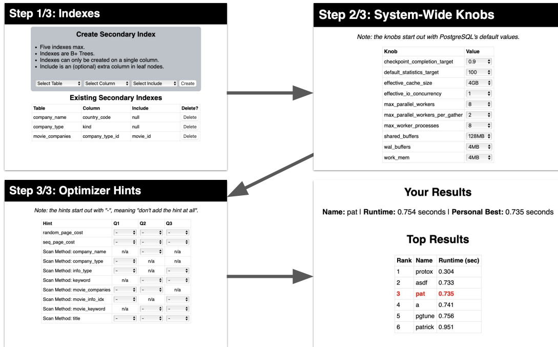
Figure 3: Demo Web UI – The figure shows the main pages in the web UI that attendees will interact with during the demo. First, they will select indexes. Second, they will select system knobs. Third, they will select query knobs (e.g., optimizer hints). Lastly, they will see their runtime on a leaderboard.
