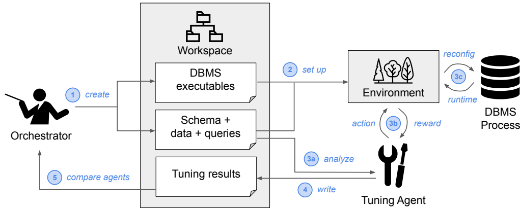
Figure 1: DB-GYM Architecture – An overview of the three components of the DB-GYM: (1) Orchestrator , (2) Tuning Agent , and (3) DBMS Process . The DB-GYM also provides two interfaces (unfilled icons in gray boxes) that these components use to interact with each other: (1) Workspace and (2) Environment . The arrows with blue labels represent the steps in the workflow when using the database gym. First, the Orchestrator creates the DBMS executable and workload files (schema, table data, and queries). Second, the Environment is initialized using these files. Third, the Tuning Agent uses the Environment to tune the DBMS. Fourth, the Tuning Agent writes the results to the Workspace. Lastly, the Orchestrator compares the results across different Tuning Agents.
