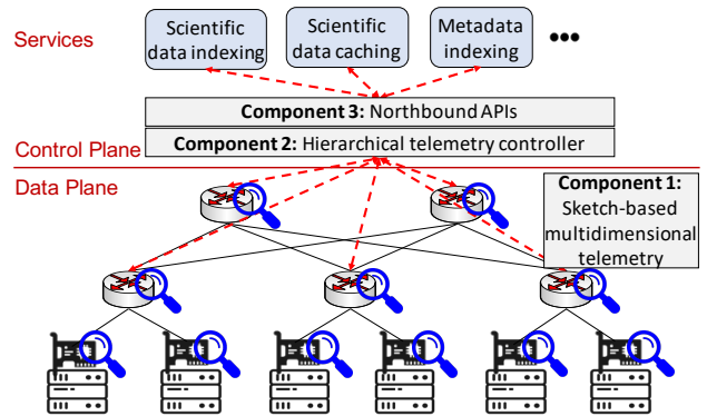
Figure 3: Overview of NSinC.
