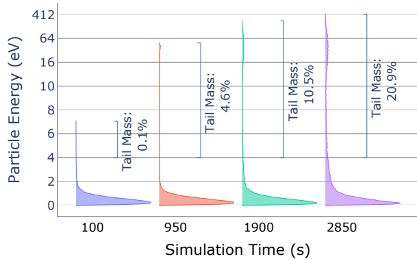
Figure 2: Distribution of particle energy during a VPIC Magnetic Reconnection simulation. Shown are the probability densities over time. The distribution changes rapidly, as energy is concentrated in a few particles.
