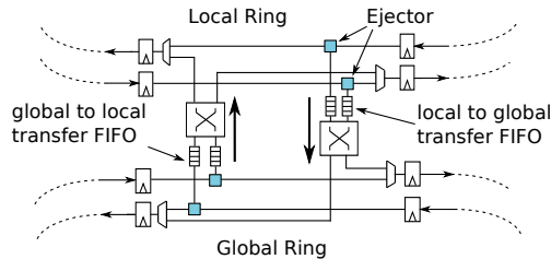
Figure 3: Bridge router.
