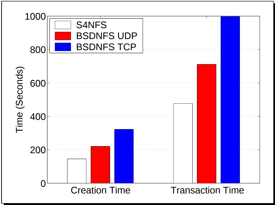
Figure 9: Postmark benchmark.
