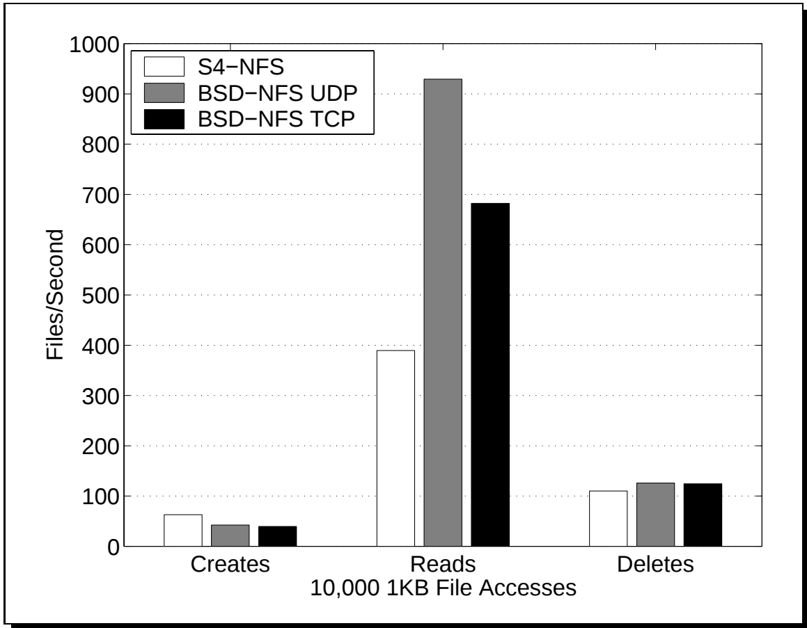
Figure 7: Small-file performance.
