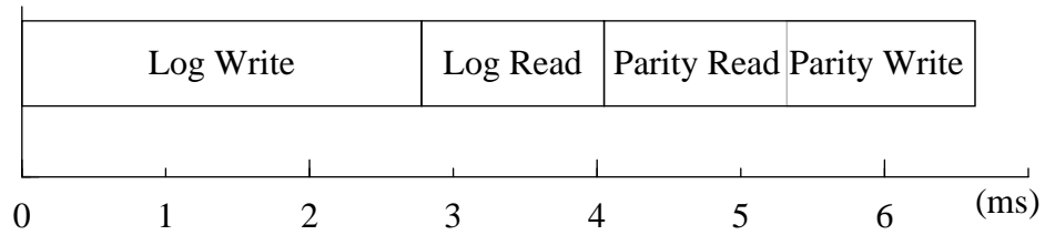
Figure 13 Parity Logging Overheads. The amortized overhead cost of extra I/Os done in our example parity logging array is shown above. The log writes contribute approximately 40% of the overhead (2.78 milliseconds), while the cylinder rate log reads, parity reads and parity writes each contribute about 20% (1.29 milliseconds). For comparison, the extra I/Os done by RAID level 5 cost nearly 35 milliseconds per small write.
