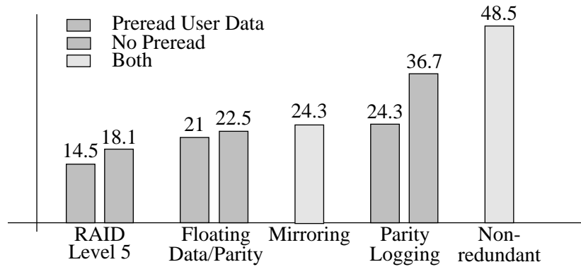
Figure 15 Model Estimates. I/Os per second per disk as predicted by the bandwidth models of section 3 and 4. These predictions assume 100% disk utilization, FIFO disk arm scheduling and an unbounded number of requestors. RAID level 5 and parity logging disk arrays both benefit substantially from not having to preread user data. Floating data and parity substantially reduces the overhead of the user preread and therefore achieves less benefit from its elimination. Mirroring and nonredundant disk arrays do not need to preread user data. Since these predictions assume 100% disk utilization, the parity logging estimates are insensitive to the degree of striping.
