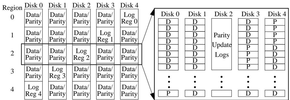
Figure 8 Block Parity Striping . Parity and data are distributed over all but one disk in each region. The remaining disk contains the parity log. A contiguous layout of parity on each disk allows efficient cylinder-rate transfers, while distribution reduces the latency of parity reintegration. The inset shows a detailed layout of a sample region.
