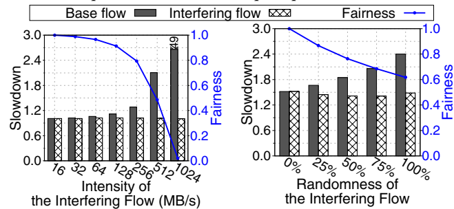
Figure 4: Effects of concurrently executing two flows with different I/O intensities on fairness.
