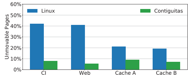
Figure 11: Unmovable 2 MB pages for Meta’s production workloads.
