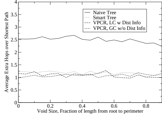
Figure 11: Performance in the presence of a void that extends radially through the network.
